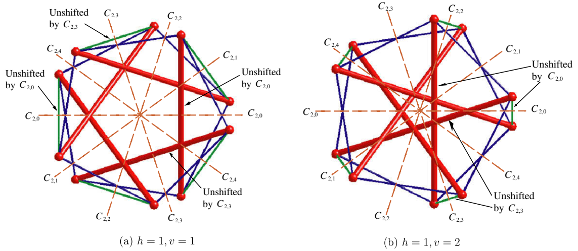
Fig. 2. Structures \mathbf{D}_n^{h,v} with n(=5) odd. One strut and one vertical cable remain unshifted by any 2-fold rotations, and all are shifted by any n -fold rotations except the identity operation.
