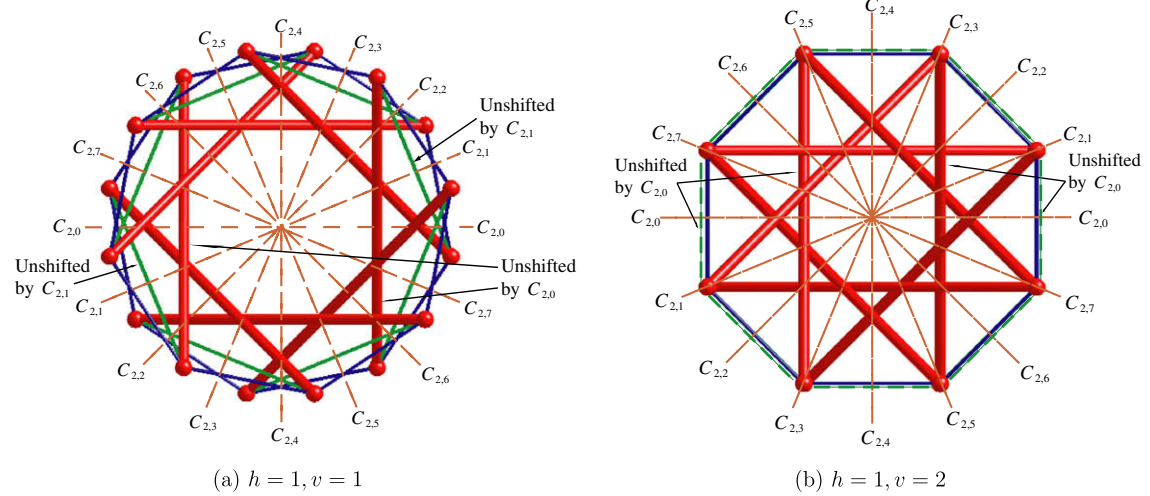
Fig. 3. Structures \mathbf{D}_n^{h,v} with n(=8) even. Two struts remain unshifted by a 2-fold rotation C_{2,2i} , and all struts are shifted by C_{2,2i+1} . For v odd, all vertical cables are shifted by C_{2,2i} , and two are unchanged by C_{2,2i+1} . For v even, two vertical cables are unshifted by C_{2,2i} , and all are shifted by C_{2,2i+1} (a) h = 1, v = 1 (b) h = 1, v = 2 .
