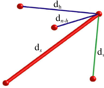
Fig. 4. A single node of prismatic tensegrity structures with dihedral symmetry. The node is connected by two horizontal cables, one vertical cable and one strut.
