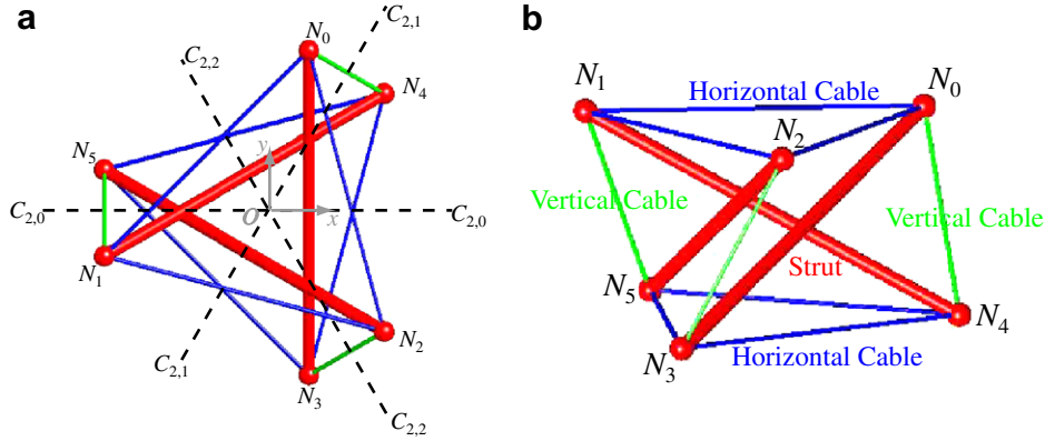
Fig. 1. The simplest three-dimensional tensegrity, a prismatic tensegrity structure with D_3 dihedral symmetry. The group D_3 has six symmetry operations: the identity, rotation by 2\pi/3 and 4\pi/3 about the z -axis, and rotation by \pi/2 about the three axes C_{2,0} , C_{2,1} , C_{2,2} . The structure consists of six nodes and six horizontal cables having a one-to-one correspondence with symmetry operations, and three vertical cables and struts having one-to-two correspondence with symmetry operations. (a) Top view. (b) Side view.
